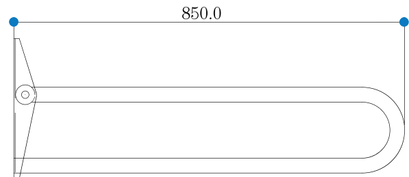
Standard Model
